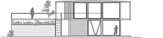
North elevation
