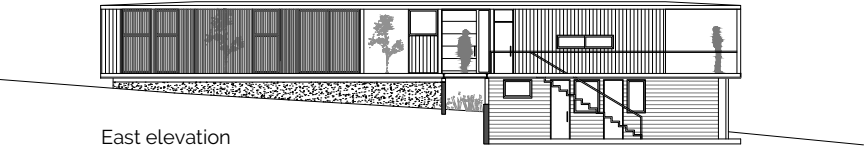
East elevation
