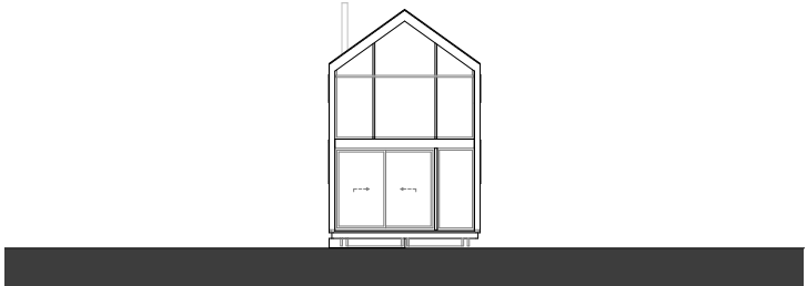
South elevation
