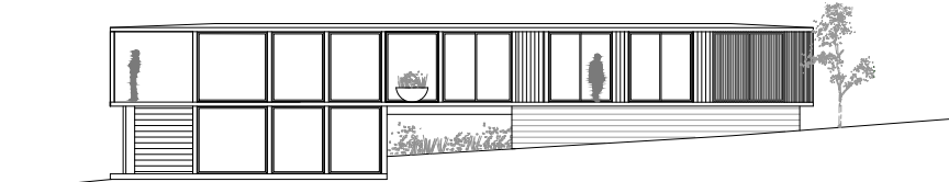
West elevation
